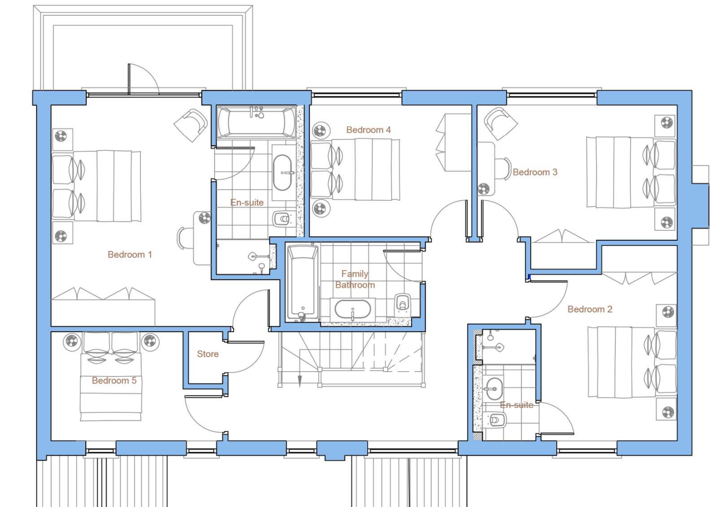
FIRST FLOOR
